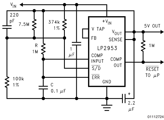
5V Regulator with Timed Power-On Reset, Snap-On/Snap-Off Feature and Hysteresis
