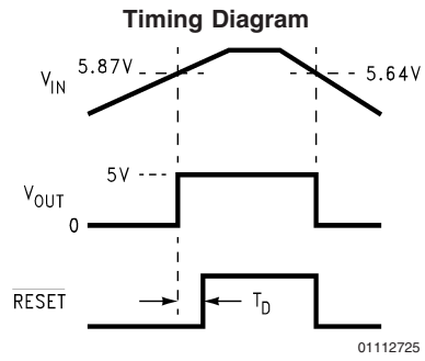
5V Regulator with Timed Power-On Reset, Snap-On/Snap-Off Feature and Hysteresis
